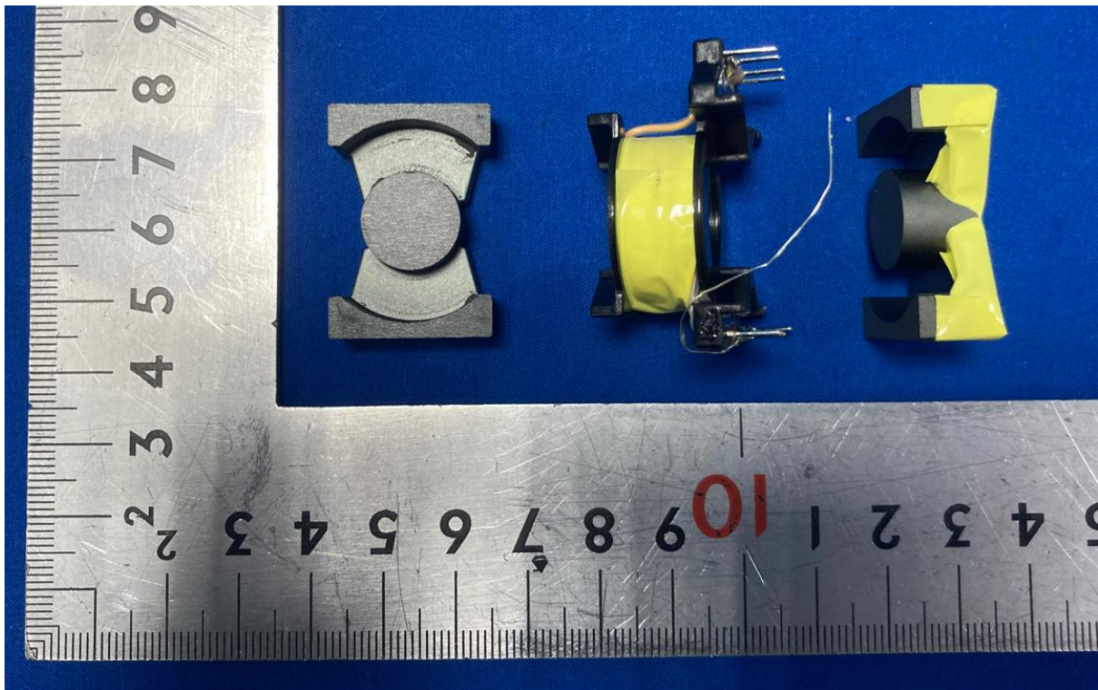
Photo -10 Internal view_1 of transformer T1
