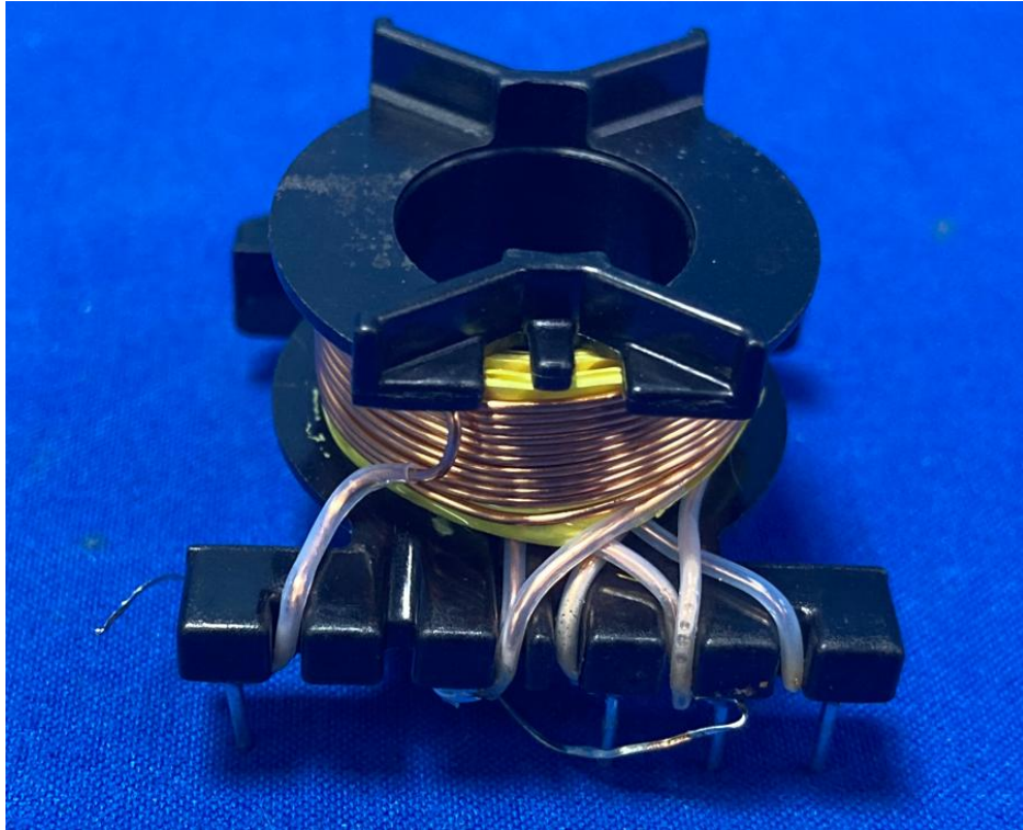
Photo -11 Internal view_2 of transformer T1
