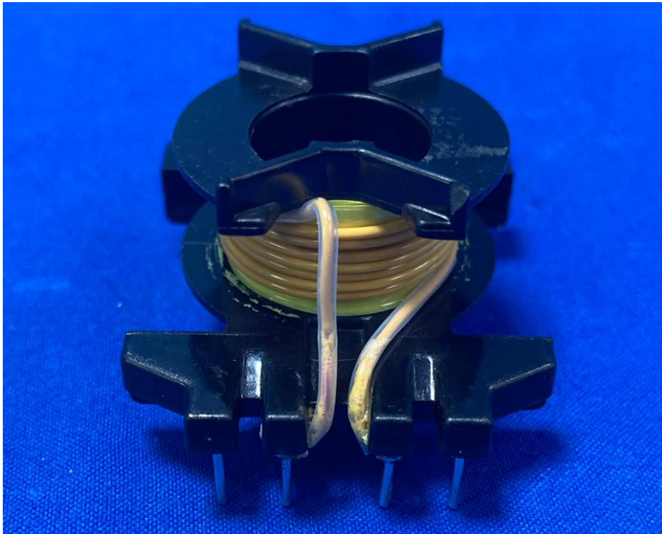
Photo -12 Internal view_3 of transformer T1
